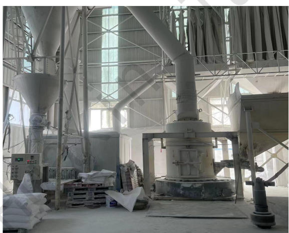
5R Raymond Grinding Mill-1 Pass Rate: 90%-99.99%
